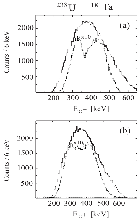
Fig. 4. a) Measured e^+ -energy spectrum from ^{238}\text{U} + ^{181}\text{Ta} collisions at a beam energy of 6.3 \times A MeV. The dotted-line histogram indicates the e^+ -contribution, multiplied by 10, which can be expected from IPC of excited states in the Ta-like nucleus (cf. fig. 3a). Both spectra are corrected for Doppler shifts, assuming an emission from the Ta-like recoils scattered in the R_{\min} range between 21.4 and 24 fm. b) The corresponding spectra obtained in the laboratory system are shown.
