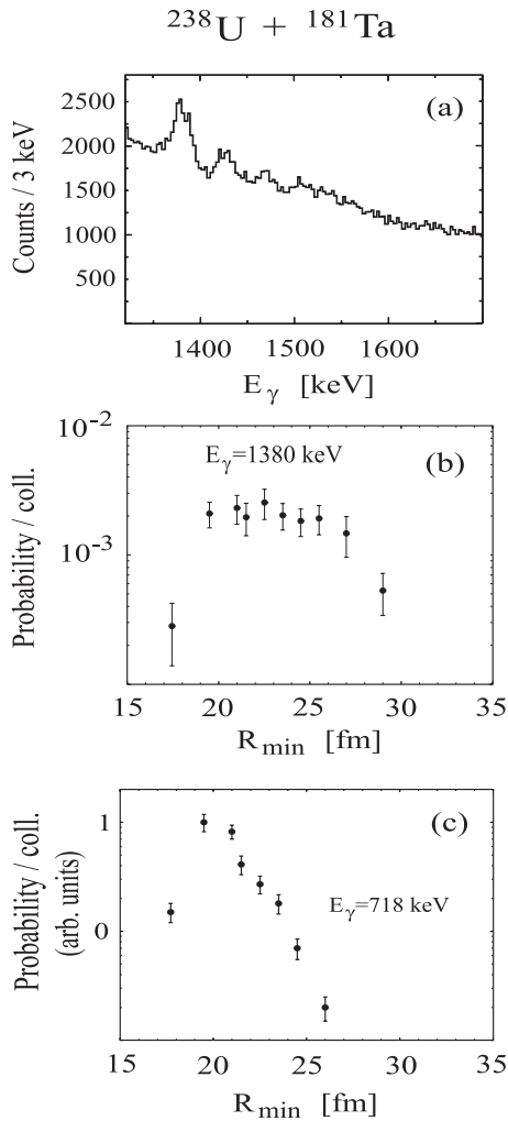
Fig. 1. a) Doppler-shift corrected \gamma -ray spectrum observed in the collision system ^{238}\text{U} + ^{181}\text{Ta} at a beam energy of 6.3 \times A MeV. Ta-like recoiling ions for rather peripheral collisions ( R_{\min} = 21.4\text{--}24 fm) are assumed to be the emitter. Several lines appear at energies below 1600 keV (see also fig.8 of ref. [12]). b) Excitation probability of the strongest \gamma -line at \sim 1380 keV as a function of R_{\min} . These data were first presented in ref. [12]. c) Excitation probability for a well known E2 \gamma -transition at 718 keV in a lower-lying rotational band in ^{181}\text{Ta} (not shown in 1a) as a function of R_{\min} .
