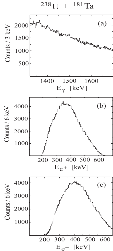
Fig. 5. a) Measured \gamma -ray spectrum, corrected for Doppler shifts, assuming an emission from the U-like ions scattered in the R_{\min} range from 19 to 29 fm. b) Measured e^+ -energy spectrum in the laboratory system for the above R_{\min} range. c) The same as in fig. 5b, but after Doppler-shift correction to the U-like scattered ions.
