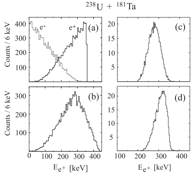
Fig. 2. Monte Carlo simulation results for energy distributions expected for e^+ and e^- emission after IPC in a nucleus with a charge number of Z = 73 and an electromagnetic transition with an energy of E_\gamma = 1380 keV and E1 multipolarity. a) Original e^+ (solid line) and e^- (dotted line) energy distributions expected in the rest frame of the emitting nucleus at the emission time. The sum of their kinetic energies has always a constant value which is given by the energy of the \gamma -transition. b) The original e^+ -energy distribution after transformation into the laboratory system to account for the Doppler shift due to the motion of the emitting ion. c) The corresponding e^+ -energy distribution in the laboratory system by taking into account the chosen momentum acceptance of the spectrometer. d) The same events as in 2c, but after an event-by-event Doppler-shift correction has been applied, utilizing the angular resolution of the setup.
