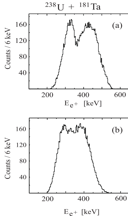
Fig. 3. Monte Carlo simulation of the e^+ -energy distribution expected from several IPC transitions in Ta ( Z = 73 ) with energies between 1250 keV and 1600 keV, as suggested by the \gamma -ray spectrum shown in fig. 1a. All the \gamma -transitions are assumed to be of pure E1 multipolarity, with the exception of the small contribution of those appearing between 1500 keV and 1600 keV for which an admixture of E2 and E0 with a mixing ratio of 1:8 [12] is taken into account. a) The e^+ -energies are corrected for Doppler shifts, assuming an emission from the Ta-like ions. b) The corresponding e^+ -energy distribution expected in the laboratory system is shown.
